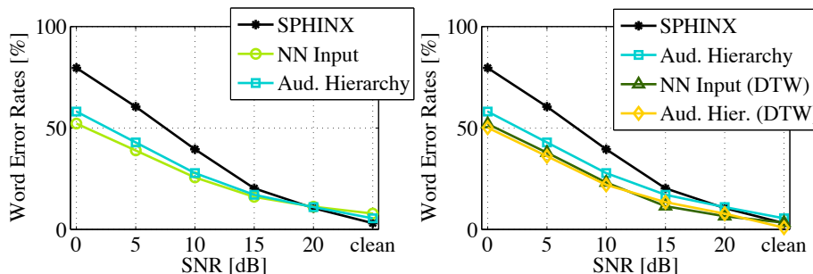
Fig. 4: Comparison of the Word Error Rates (WER) between the proposed system and Sphinx-4 in the presence of babble noise. Left: Recognition performance at the input and output of the hierarchy. Right: Recognition performance when Dynamic Time Warping is used to scale the signals.
