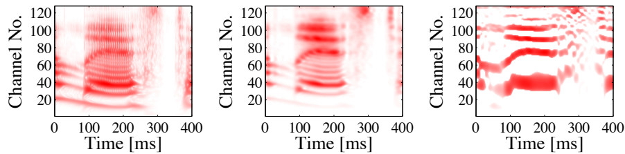
Fig. 2: Overview of the preprocessing step for the word "list" spoken by a female american speaker. Left: response of the basilar membrane. Center: after a low-pass filtering over the time and a preemphasis. Right the harmonic structure has been removed using a filtering along the frequency axis.
